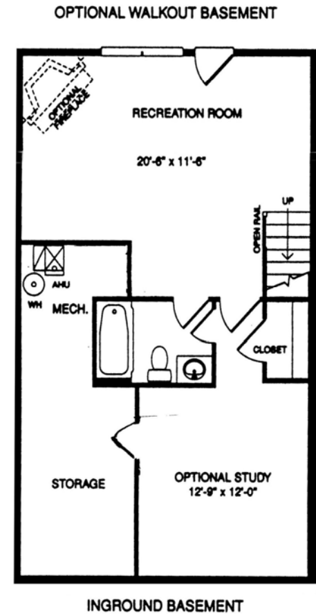
Lower Level Plan
